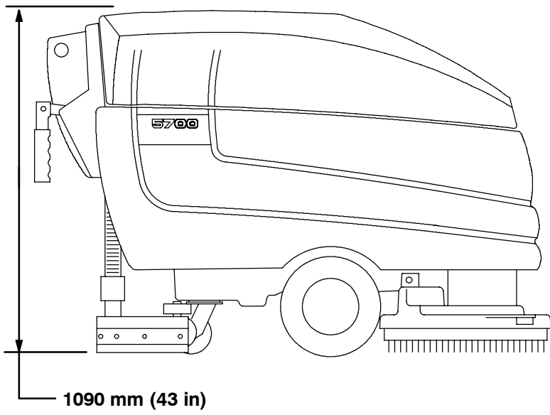
MACHINE DIMENSIONS
